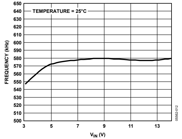
Figure 12. Oscillator Frequency vs. Input Voltage
